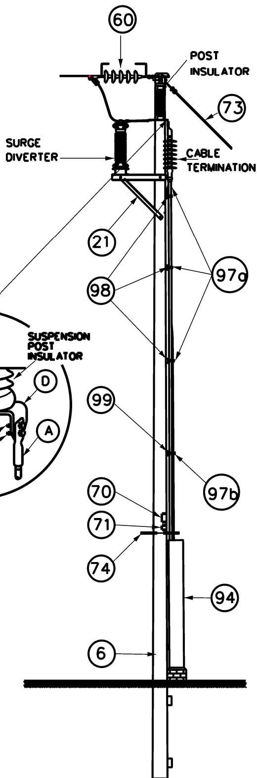
SIDE ELEVATION
